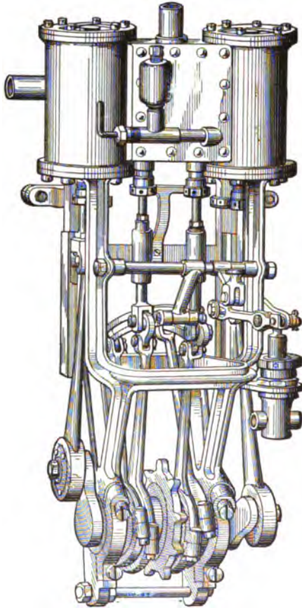
FIG. 246.—The "Locomobile" Steam Carriage Engine.
